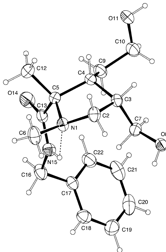
Figure 2. ORTEP plot of alcohol 19 . Ellipsoids are drawn at 30% probability level.
