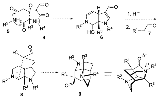
Scheme 2. General strategy.
