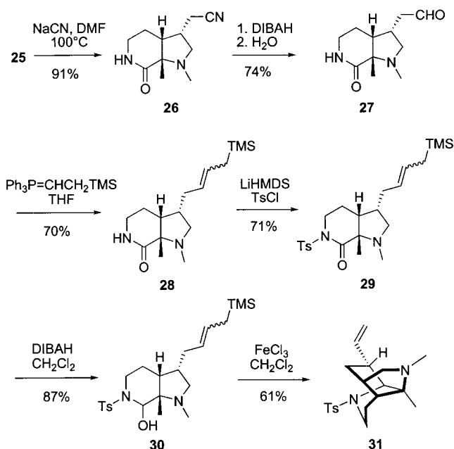
Scheme 6. Synthesis of sarain A model 31 by an allylsilane strategy. [2]
