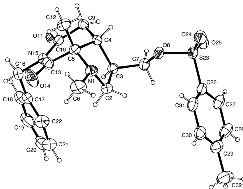
Figure 1. ORTEP plot of tosylate 17 . [13] Ellipsoids are drawn at 30% probability level.
