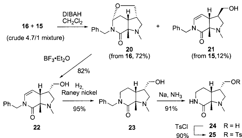
Scheme 5. Selective imide 16 reduction.
