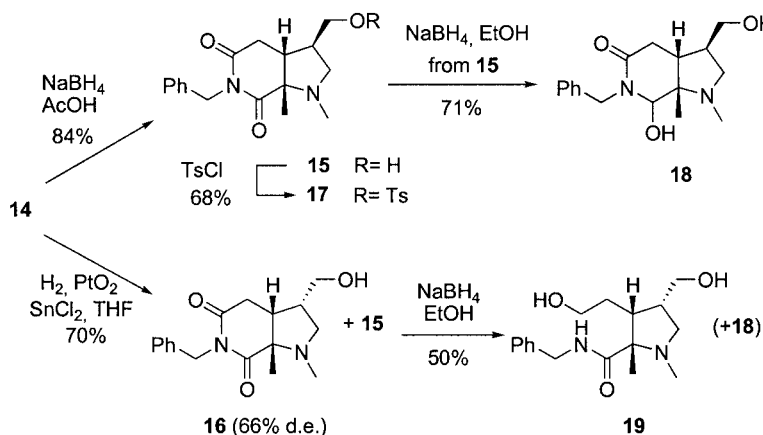
Scheme 4. Reduction studies on intermediate 14 .
