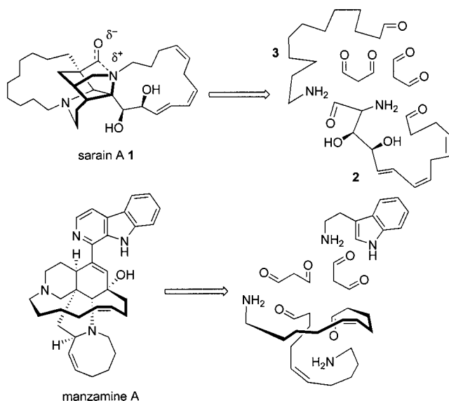
Scheme 1. Proposed biogenetic pathway.
