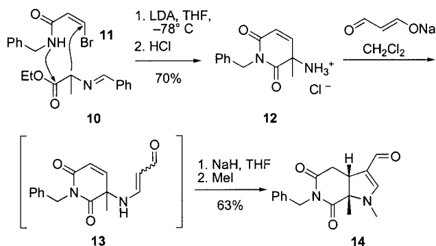
Scheme 3. Short route to a diazabicyclo[4.3.0]nonane system.
